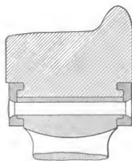
Fig. 4562. Double Lip Retaining Ring with 4 3/8-in. Shrink Base.
